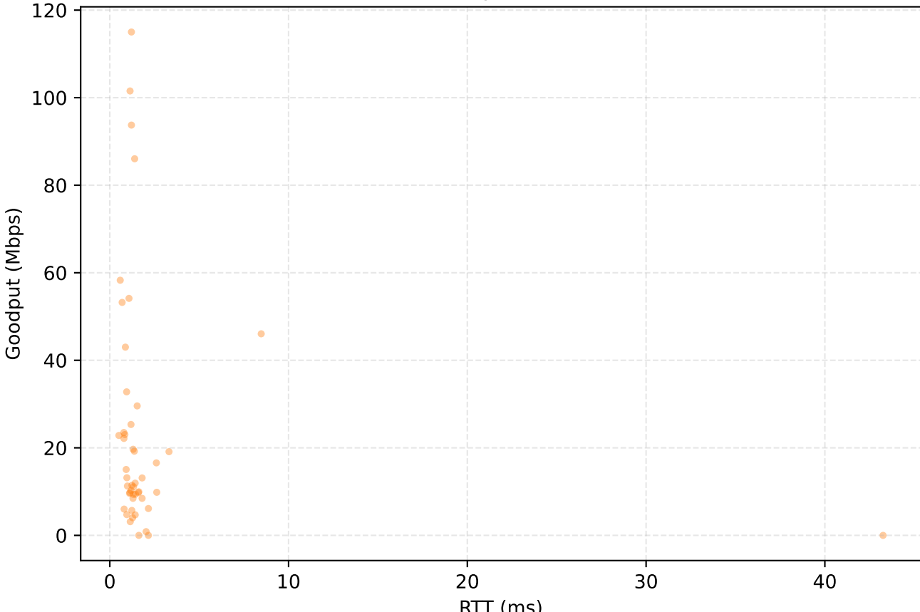
Q2 - RTT vs Goodput [102.214.66.39]
