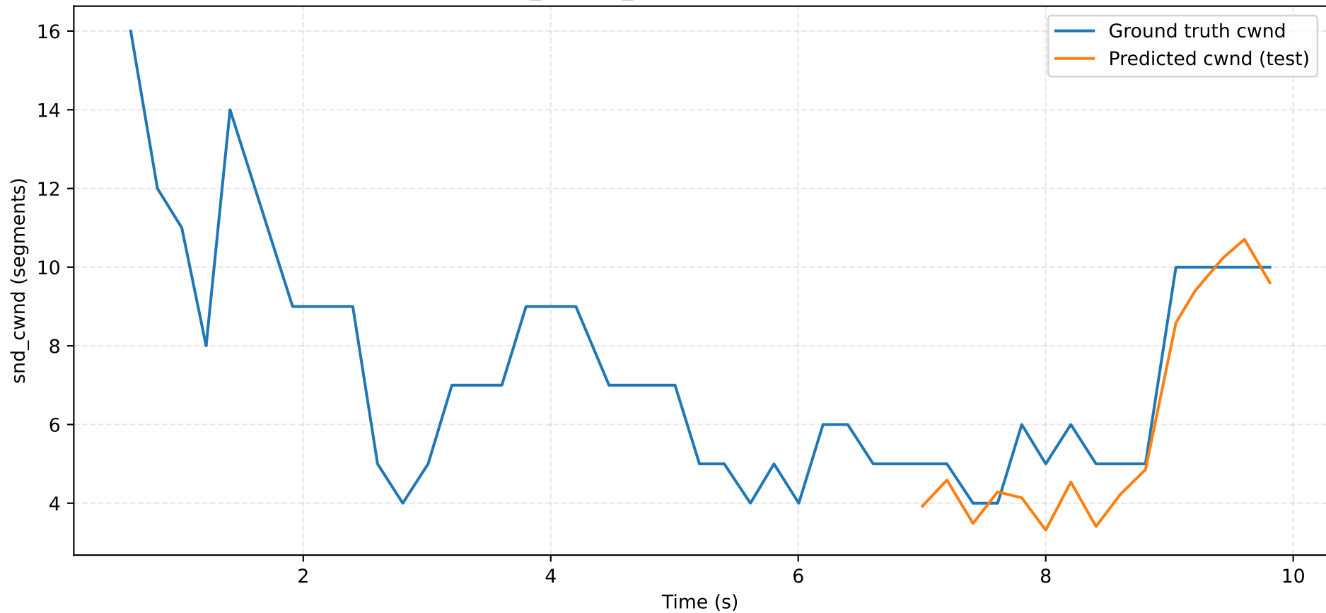
Trace trace_0 - snd_cwnd ground truth vs prediction
