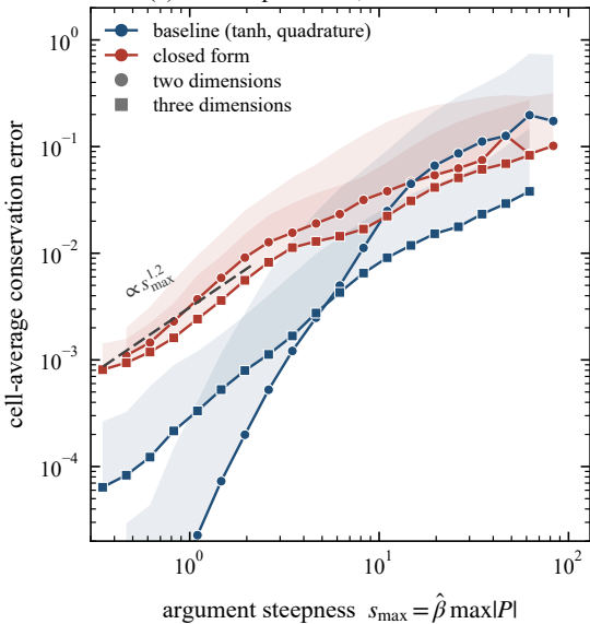
(a) one steepness law, both dimensions
