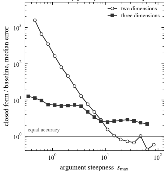
(b) the accuracy penalty closes with steepness
