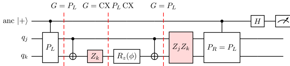
Figure 1: One bond of the ZZ layer, U = CX(j, k) R_z^{(k)}(\phi) CX(j, k) = \exp(-i\frac{\phi}{2} Z_j Z_k) , bracketed by a coherent Pauli check. Dashed slices show the check image G propagated to each time; the shaded boxes are the two faults that no valid flavor can see.
