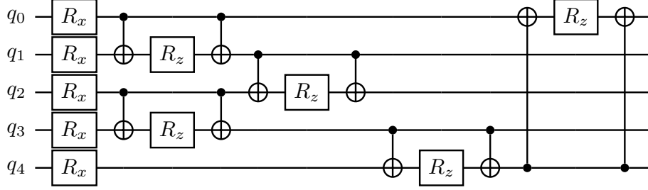
Figure 6: One Trotter step of the payload on the five-qubit ring: R_x(\theta) on every qubit, then the ZZ layer with bonds (0, 1), (2, 3), then (1, 2), (3, 4), then the closing bond (4, 0), each compiled as CX_{jk}R_z^{(k)}(\phi)CX_{jk} ; ten noisy CX gates per step ( g_p = 10 ).
