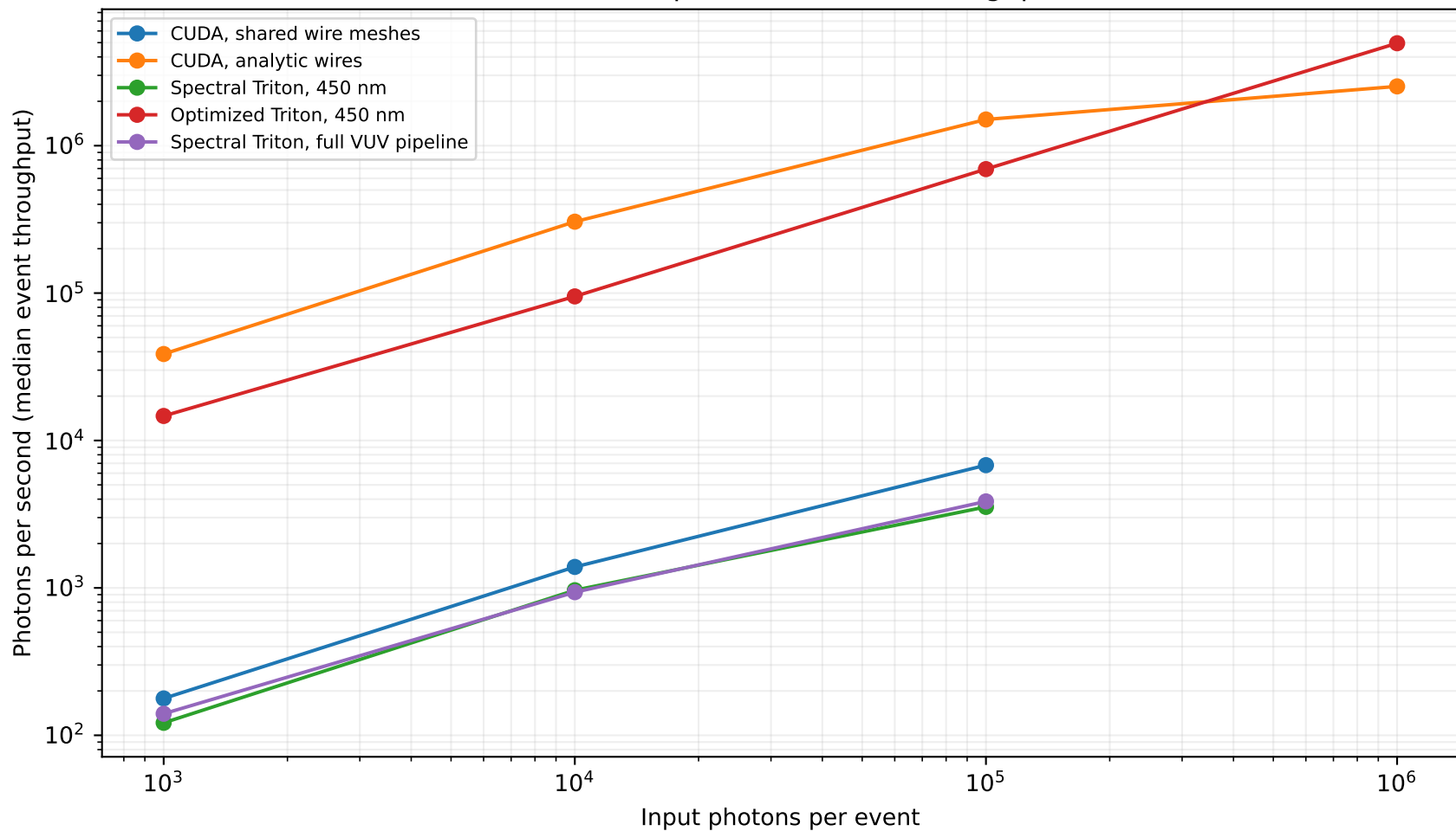
Local A100 optical simulation throughput
