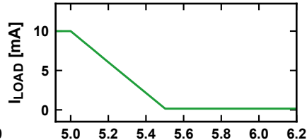
(c) Overshoot
