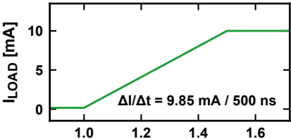
(a) Undershoot
