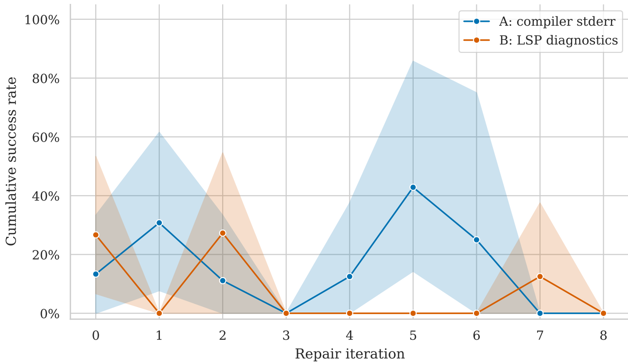
Cumulative success rate vs. repair iteration (shaded = 95% CI)
