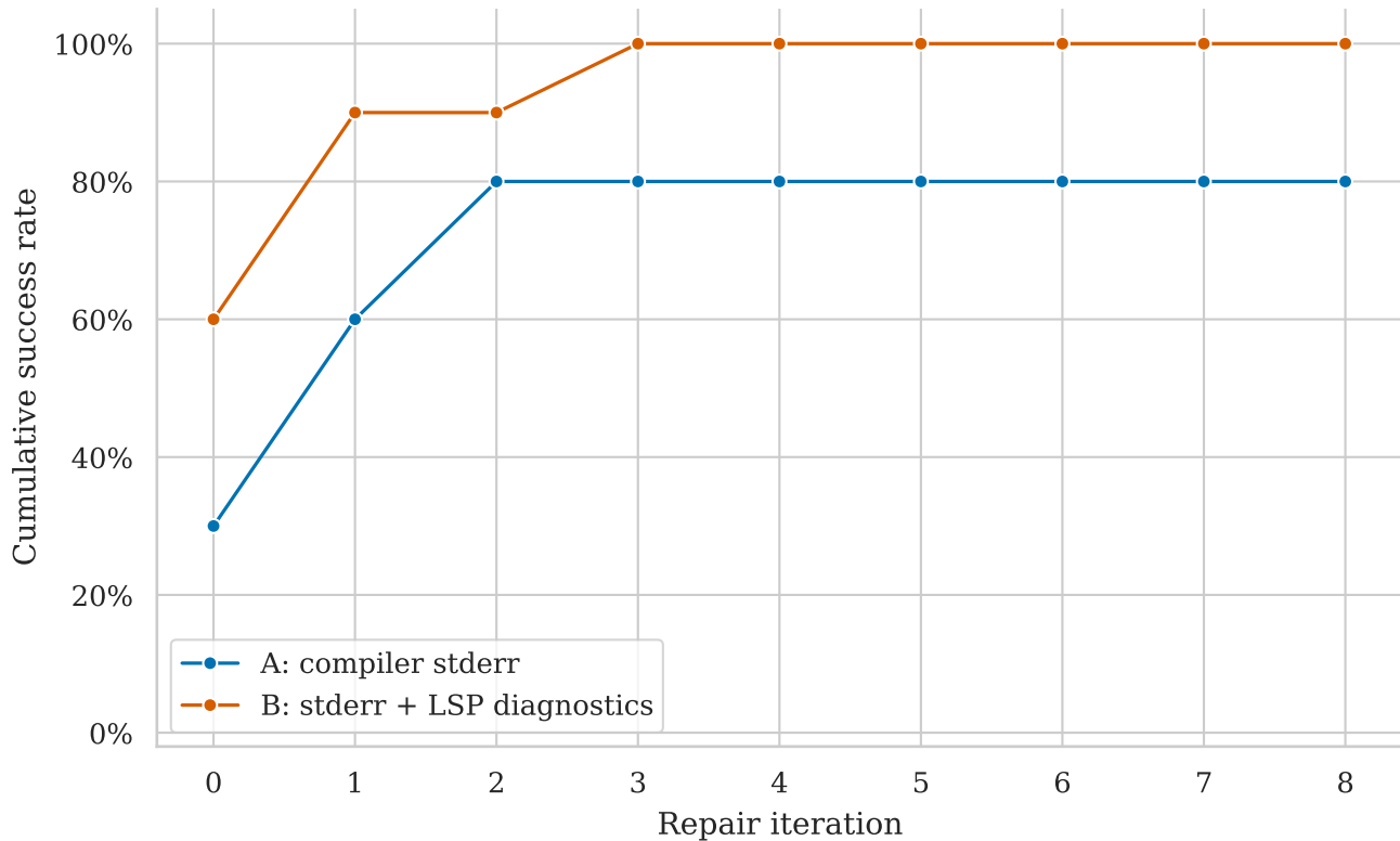
Cumulative success rate vs. repair iteration
