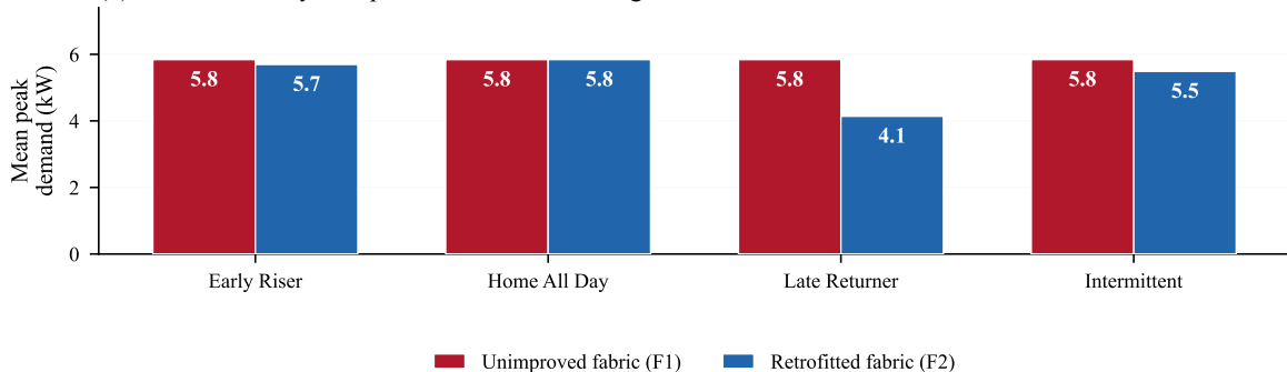
(b) Peak demand by occupant × fabric · W2 design cold
