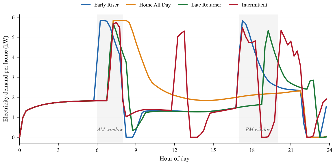
(a) Daily demand profile · W2 design-cold day, F1 unimproved fabric
