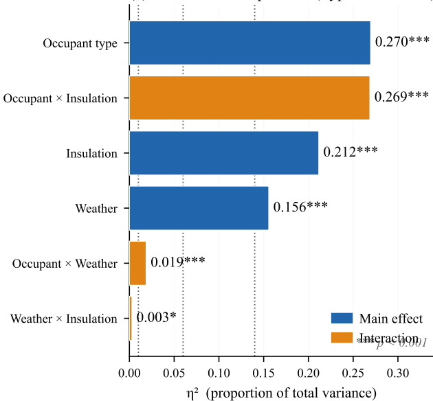
(a) Variance decomposition (Type-II ANOVA)
