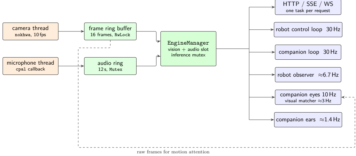
Figure 3: Runtime view. Orange: OS threads. Blue: Tokio tasks. Green: shared state. Two handles force the thread boundary on the left: a nokhwa camera and a cpal input stream are not Send , so each is owned by a dedicated thread that pushes into a shared ring; everything else is asynchronous. On the right, every consumer reaches the model through a single EngineManager , whose inference mutex serialises forward passes so that concurrent requests cannot multiply the GPU working set (Section 8).
