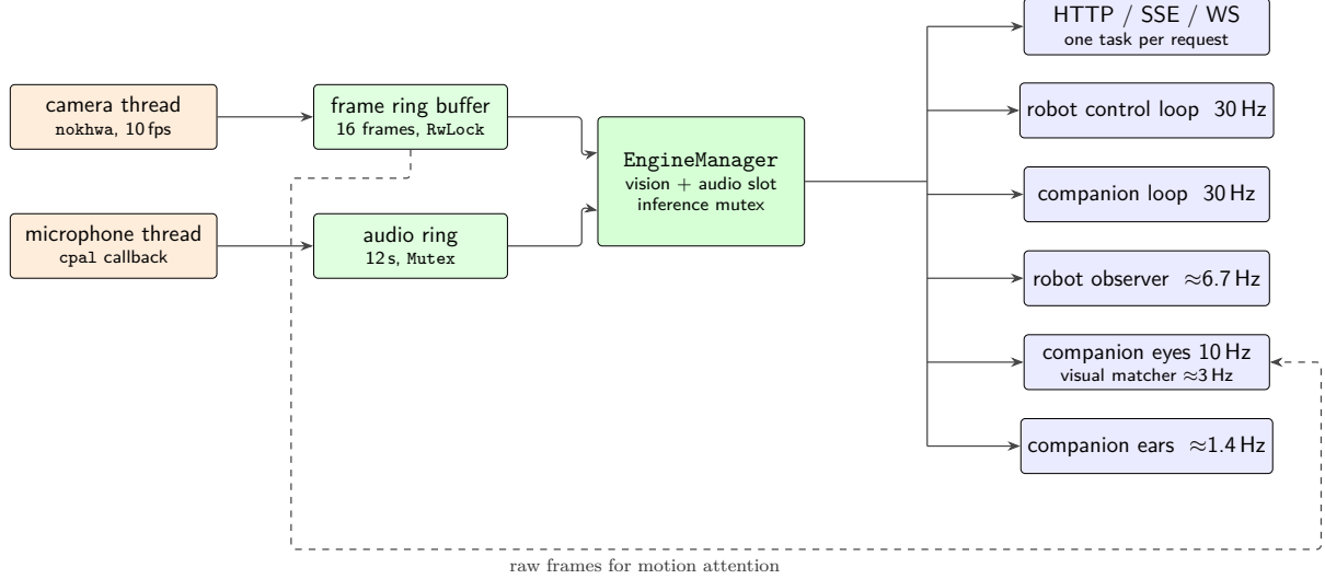
Figure 3: Runtime view. Orange: OS threads. Blue: Tokio tasks. Green: shared state. Two handles force the thread boundary on the left: a nokhwa camera and a cpal input stream are not Send , so each is owned by a dedicated thread that pushes into a shared ring; everything else is asynchronous. On the right, every consumer reaches the model through a single EngineManager , whose inference mutex serialises forward passes so that concurrent requests cannot multiply the GPU working set (Section 8).
