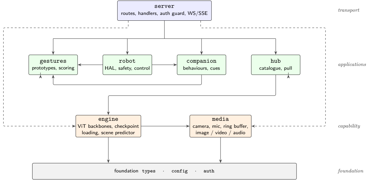
Figure 2: Module dependencies; arrows point from a module to what it uses, and dashed arrows are the two that skip a layer. Application modules depend on engine and media but never on server , so the same perception and control code is reachable from the CLI, the HTTP API, and the tests without a running daemon.
