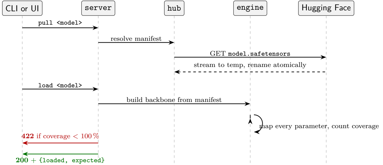
Figure 5: Pulling and loading. The runtime never serves a partially loaded model: coverage below 100 % is an error carrying the count and the first missing tensor names, not a warning in a log.
