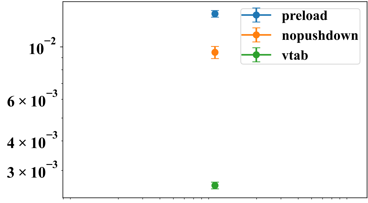
locOrder
