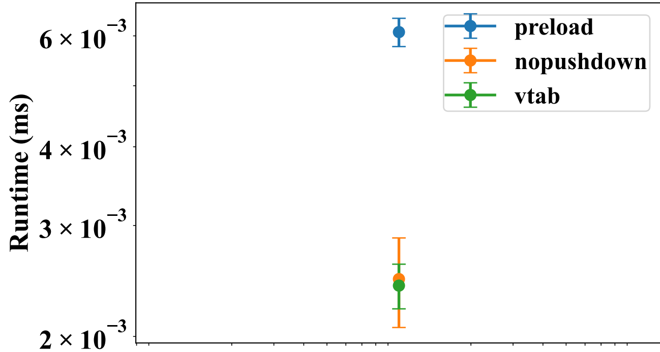
locFull
