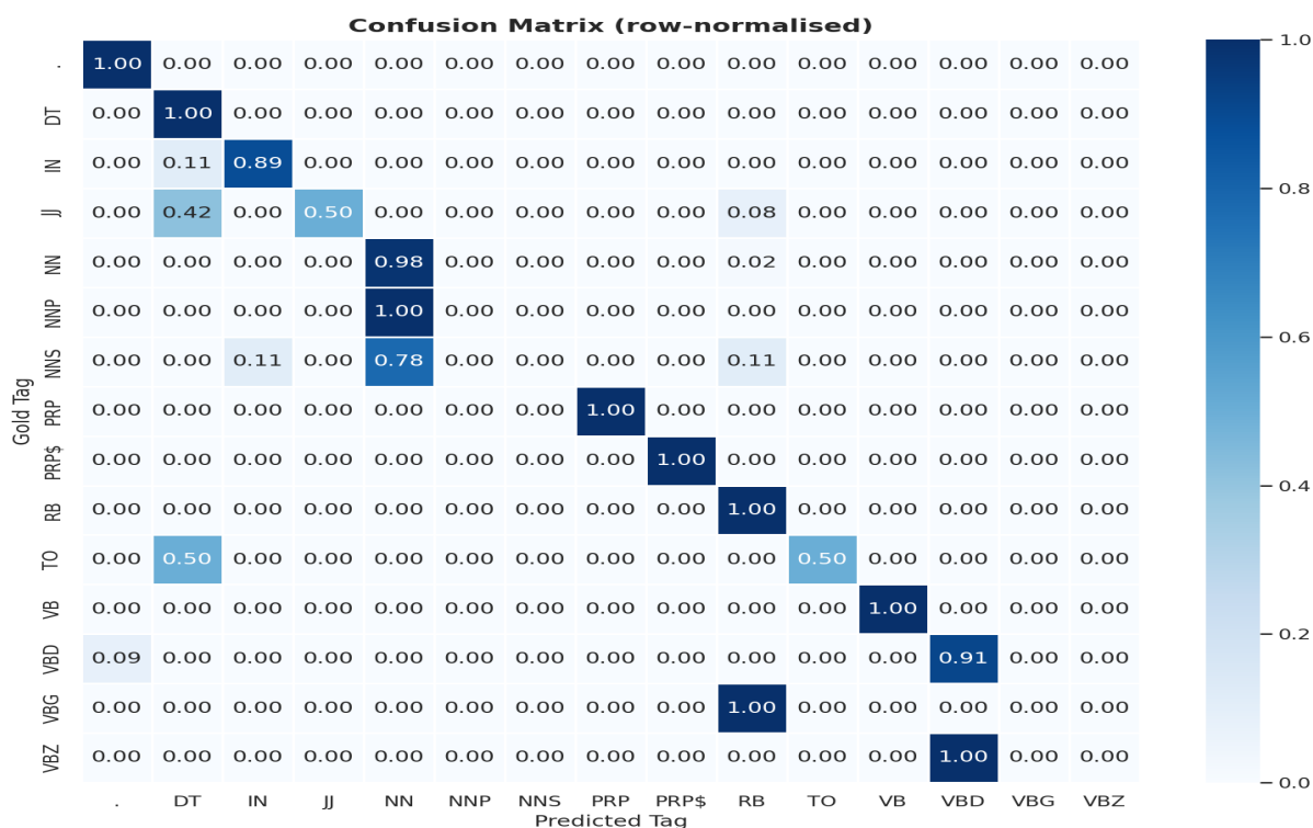
Figure 1: Confusion Matrix (row-normalised). Each cell shows the fraction of gold-tag tokens (row) predicted as each tag (column). Diagonal values represent per-tag recall.
