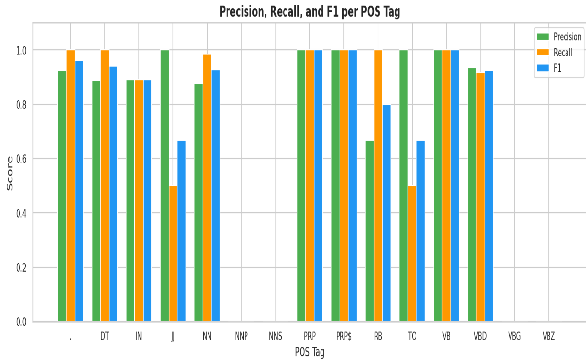
Figure 3: Precision, Recall and F1 per POS Tag. Grouped bars allow a direct comparison of all three metrics.
