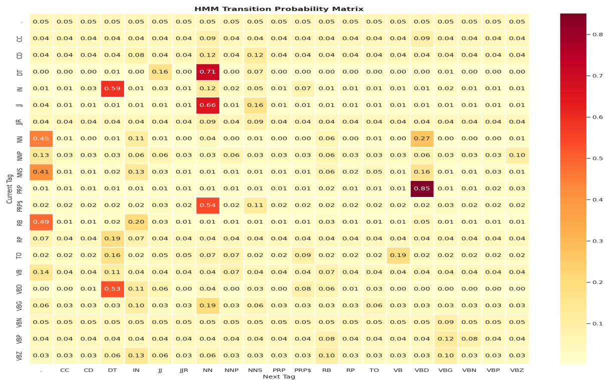
Figure 4: HMM Transition Probability Matrix. Cell (i, j) shows the smoothed probability of transitioning from tag i to tag j .
