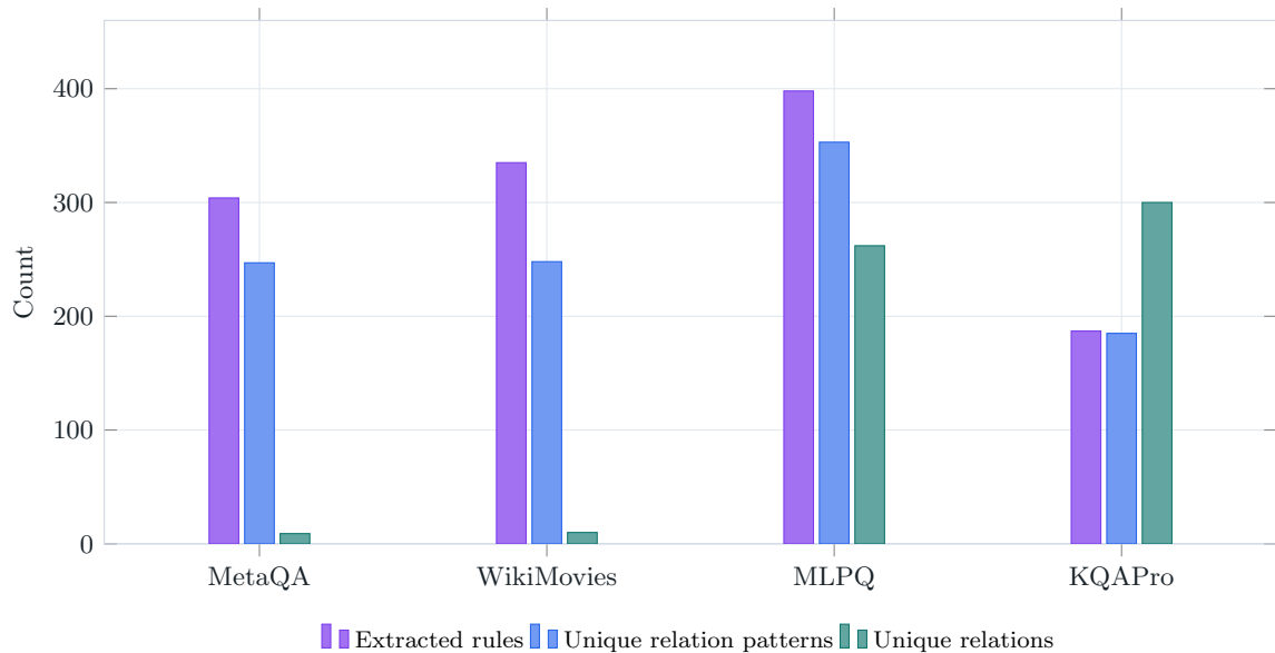
Offline grammar extraction statistics
