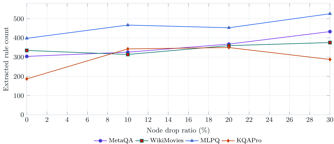
Offline HRG rule count under node deletion
