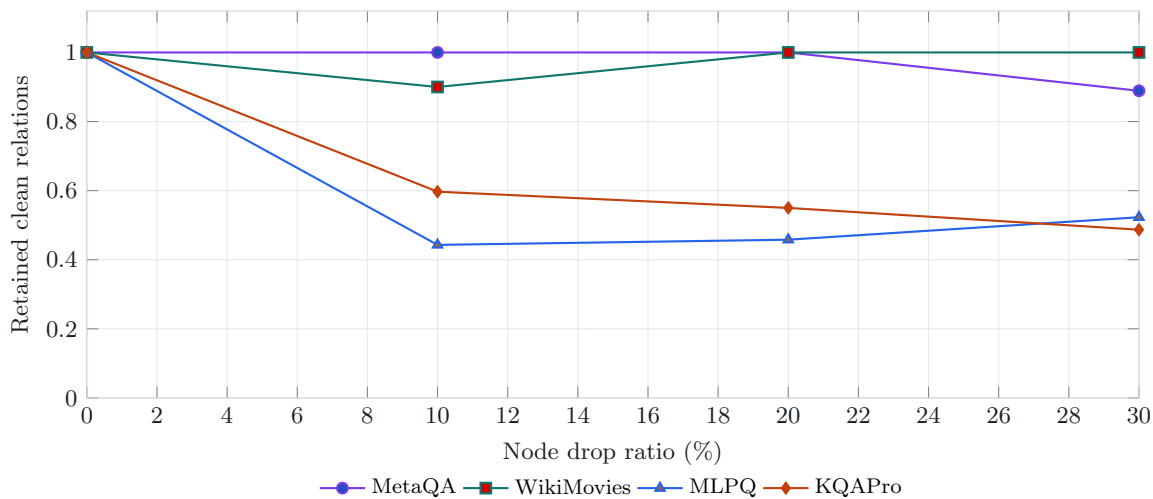
Relation vocabulary retention under node deletion
