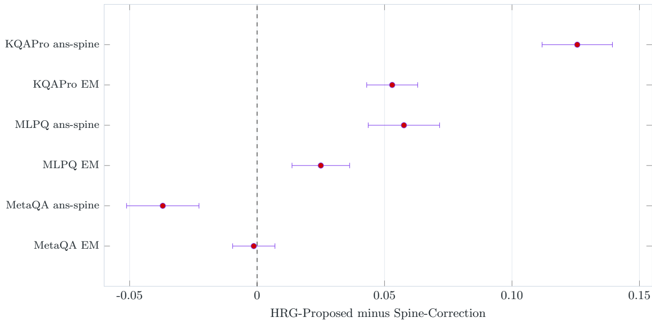
Paired bootstrap 95% CI for HRG hard-case effects
