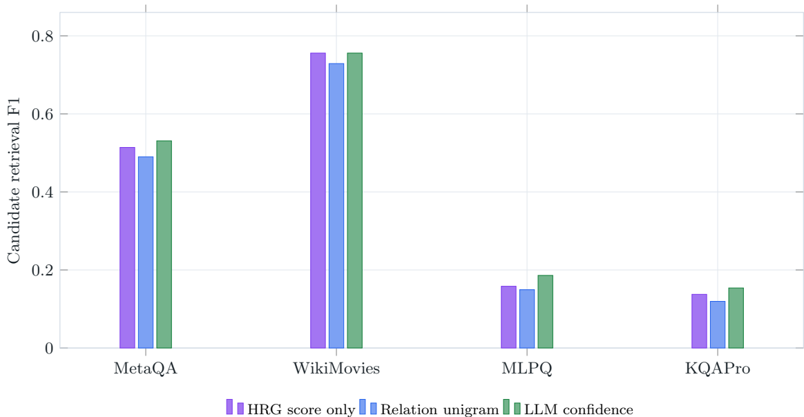
Candidate-level prior pilot: HRG score vs relation unigram
