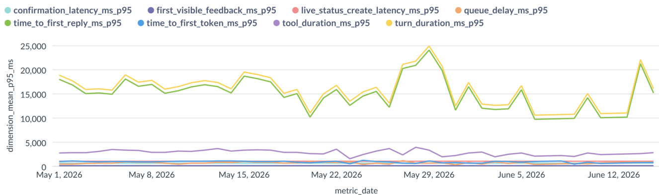
[SYNTHETIC ONLY] P95 performance trends
