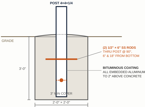
DETAIL 4 · FOOTING & COLUMN EMBEDMENT
