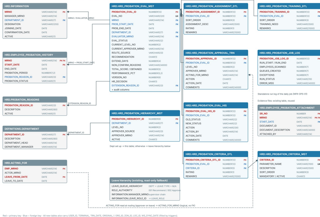
Probation Evaluation – ER Diagram (DB Structure)
