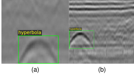
Fig. 1. Hyperbola samples.
