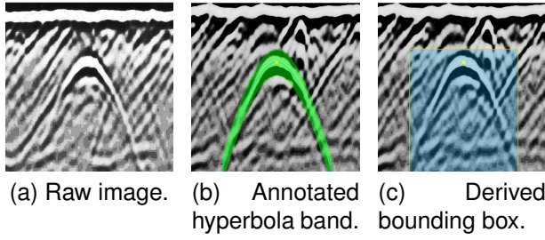
Fig. 3. Example of a hyperbola sample: the raw image, the annotated hyperbola band, and the bounding box derived from the band boundary.
