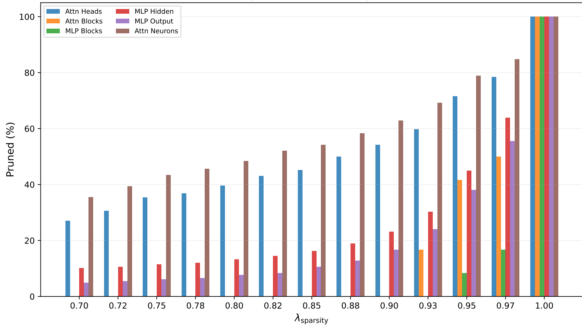
Component-level Pruning - IOI
