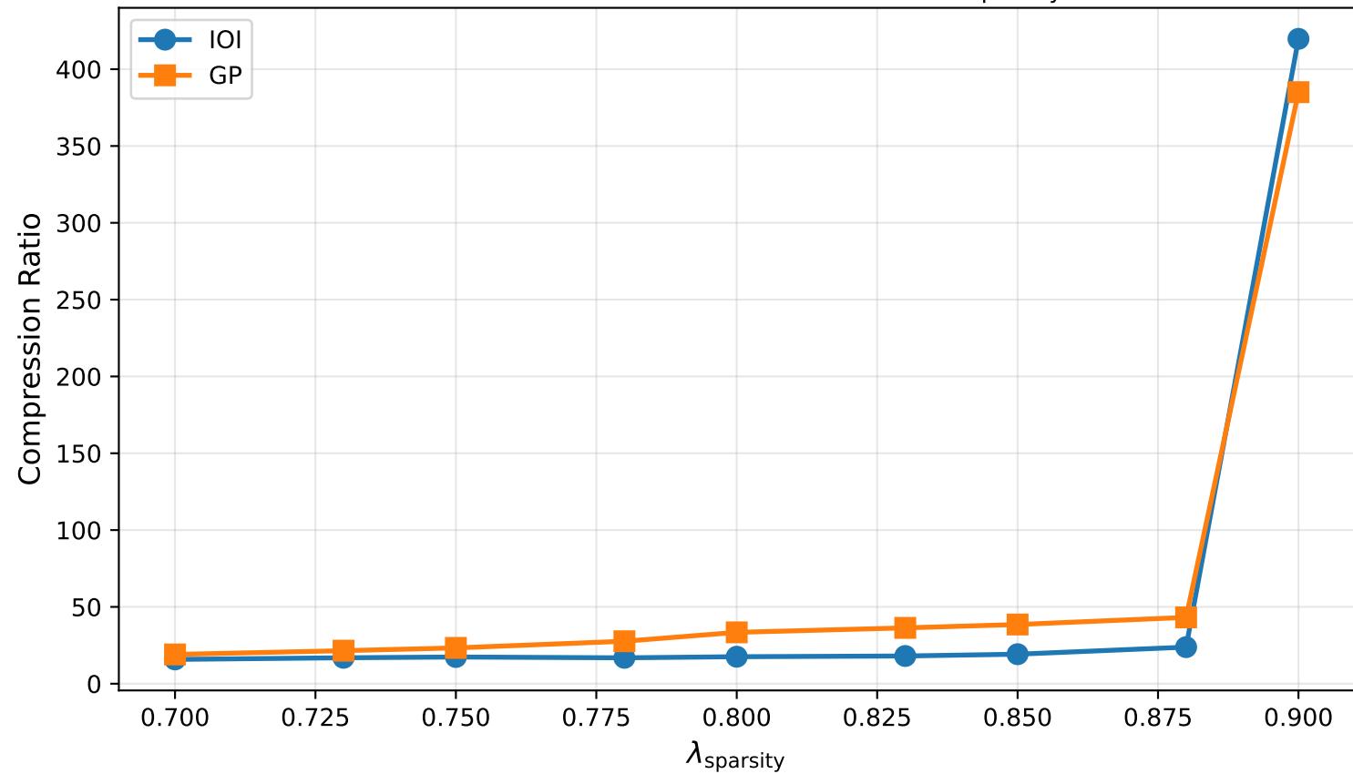
Llama-3.1-8B: Compression vs. \lambda_{\text{sparcity}}
