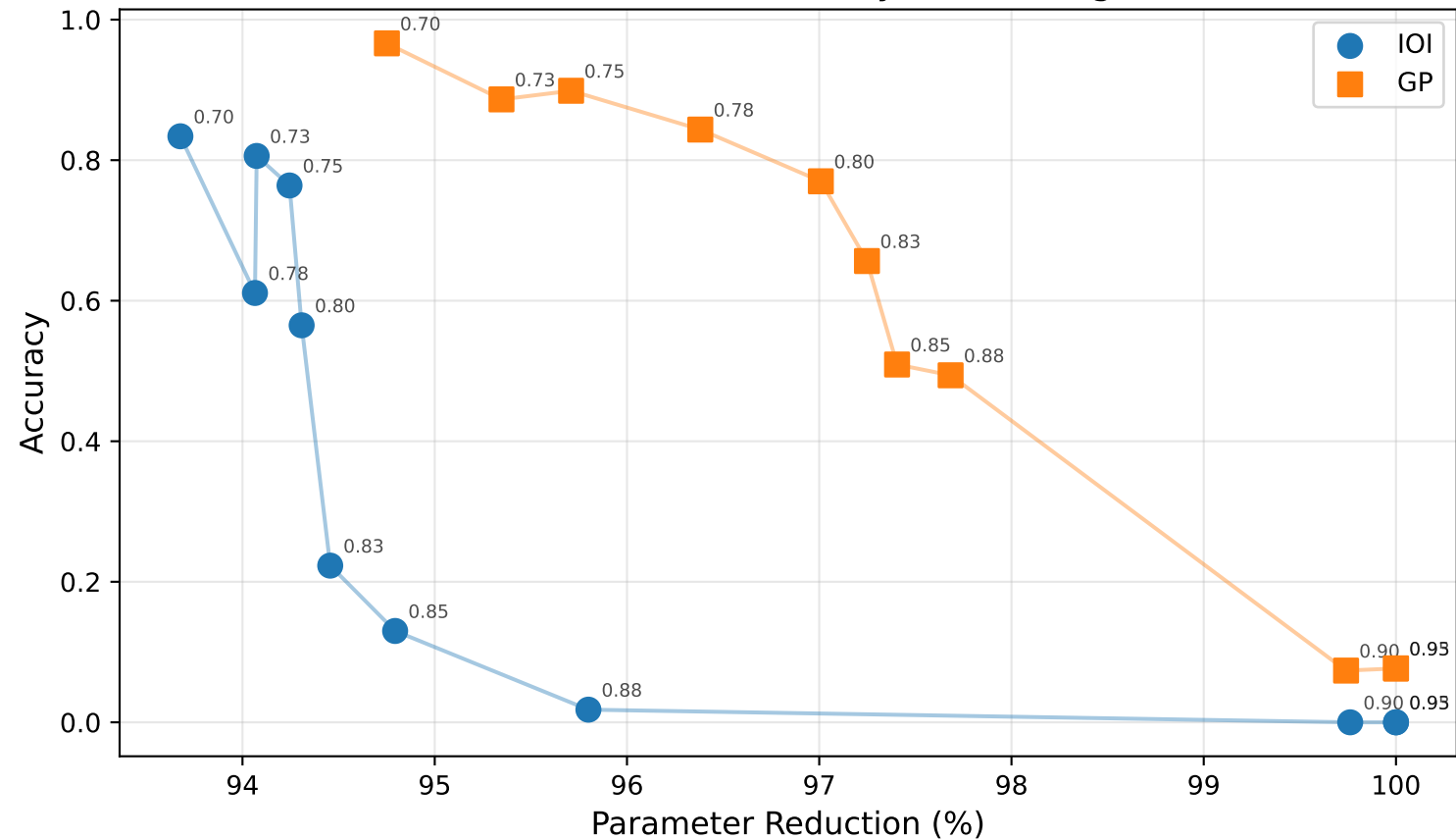
Llama-3.1-8B: Accuracy vs. Pruning
