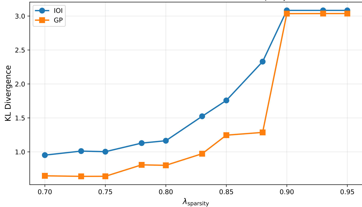
Llama-3.1-8B: KL Divergence vs. \lambda_{\text{sparse}}
