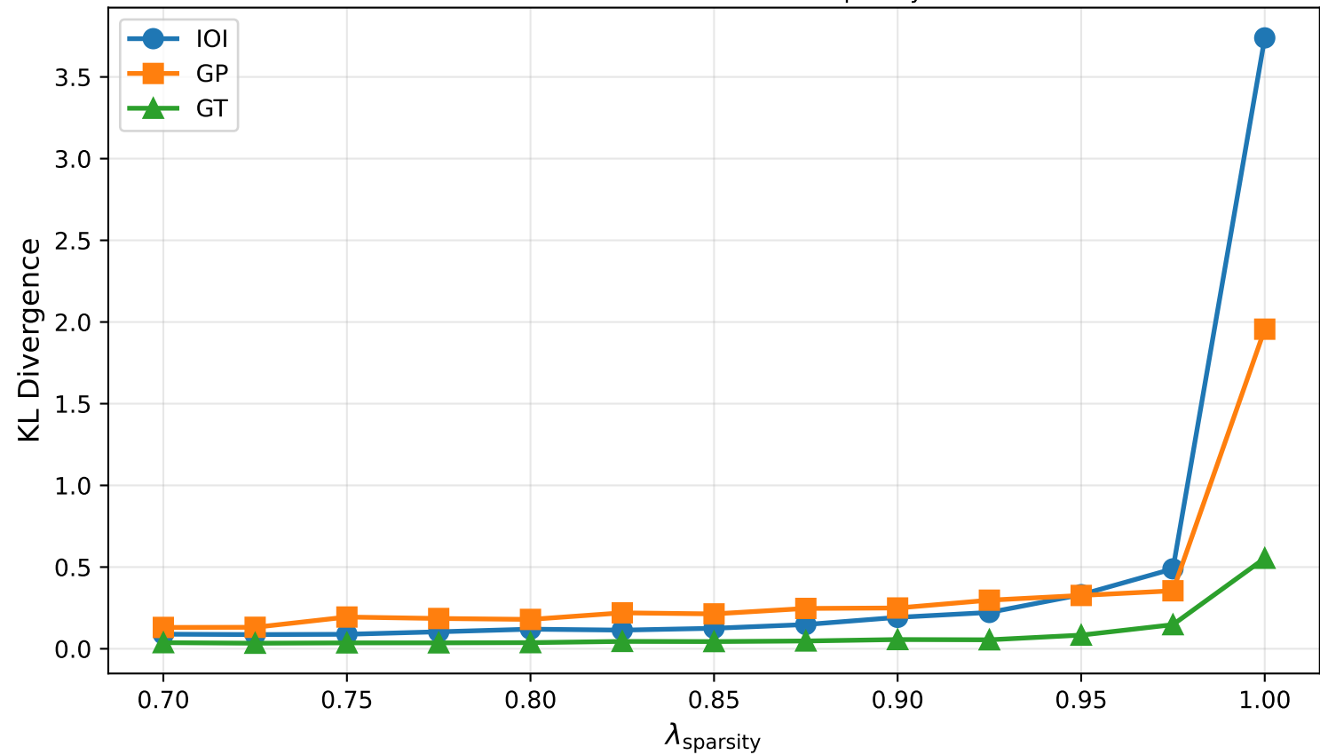
KL Divergence vs. \lambda_{\text{sparsity}}
