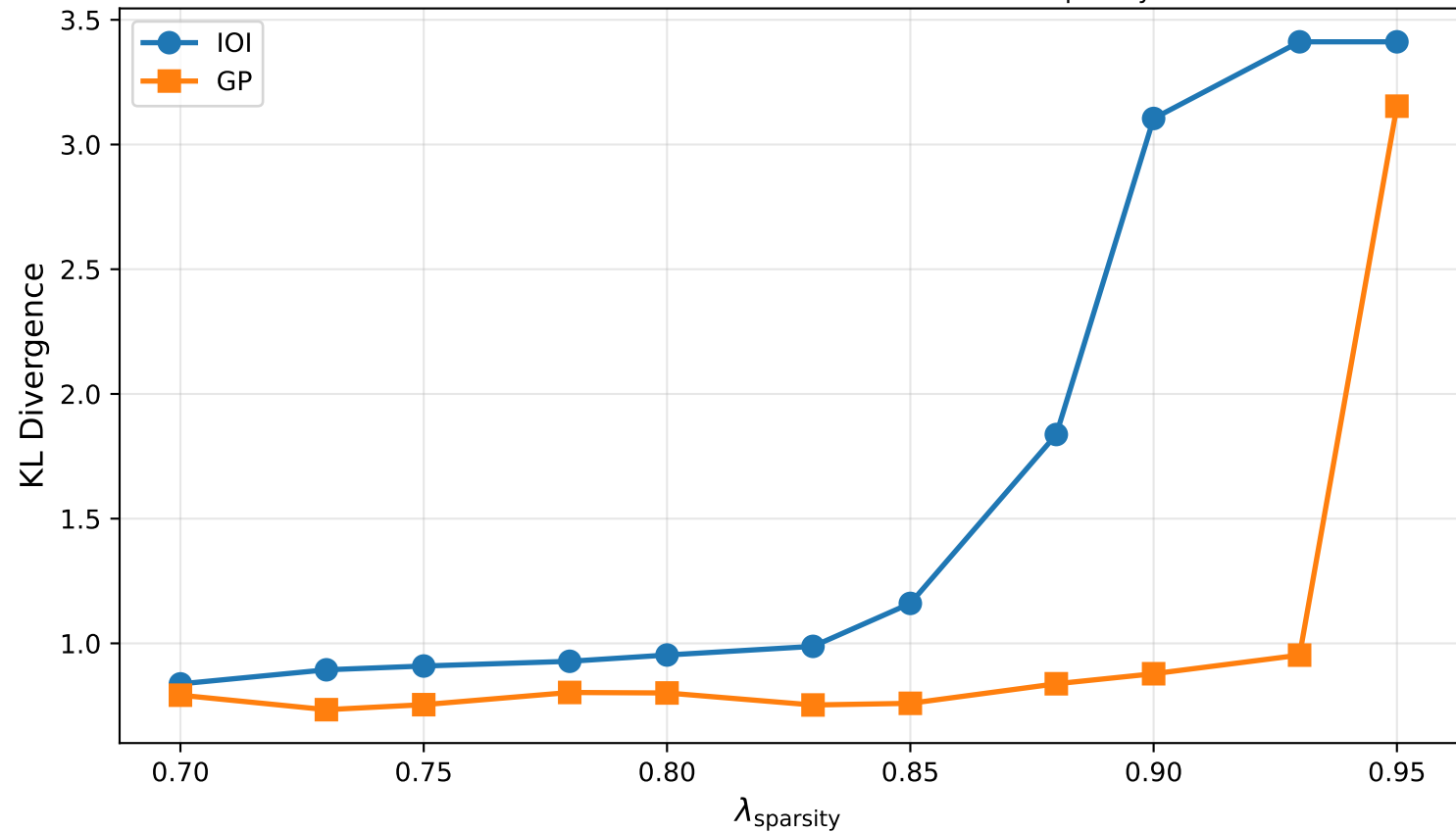
Llama-3.2-1B: KL Divergence vs. \lambda_{\text{sparcity}}
