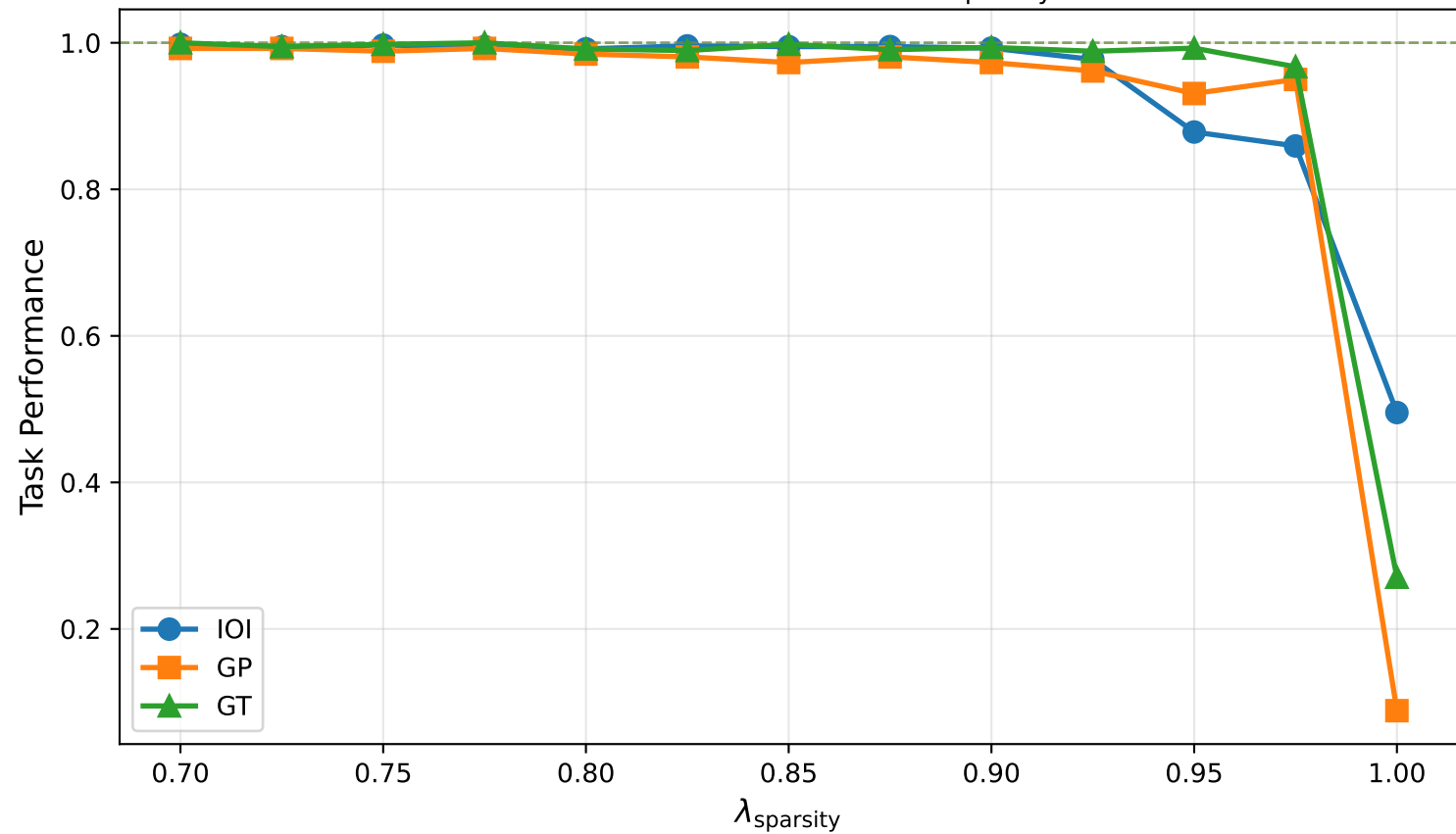
Task Performance vs. \lambda_{\text{sparsity}}
