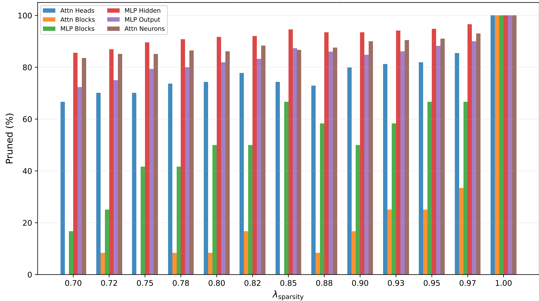
Component-level Pruning - GP
