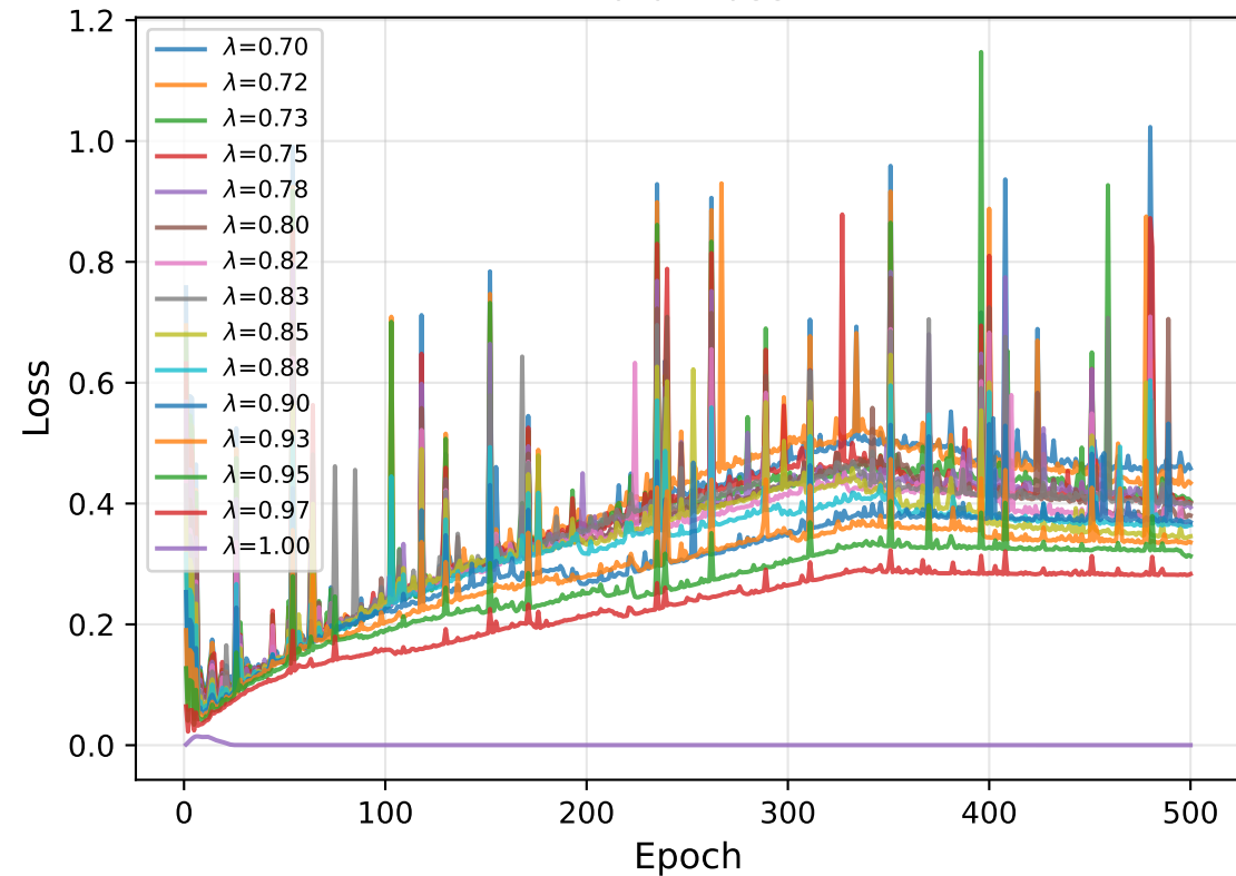
Total Loss
