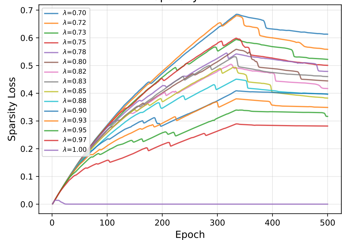
Sparsity Loss
