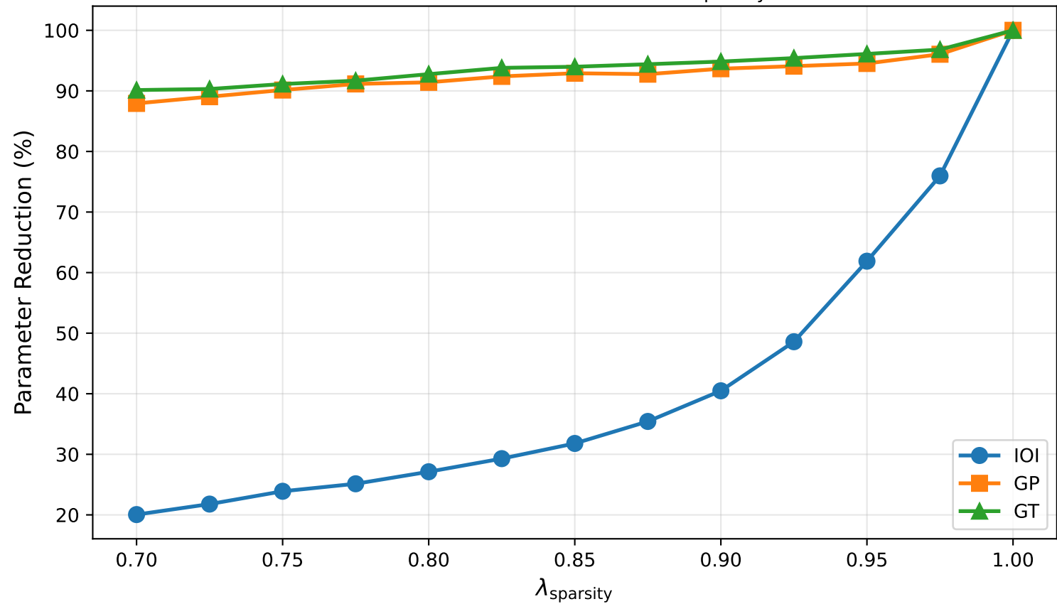
Pruning Reduction vs. \lambda_{\text{sparsity}}
