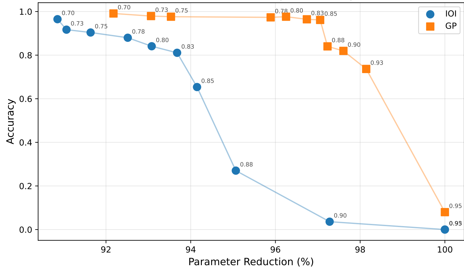
Llama-3.2-1B: Accuracy vs. Pruning
