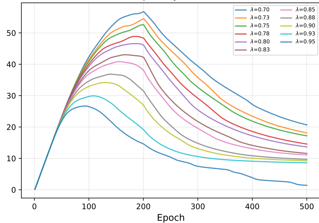
Sparsity Loss
