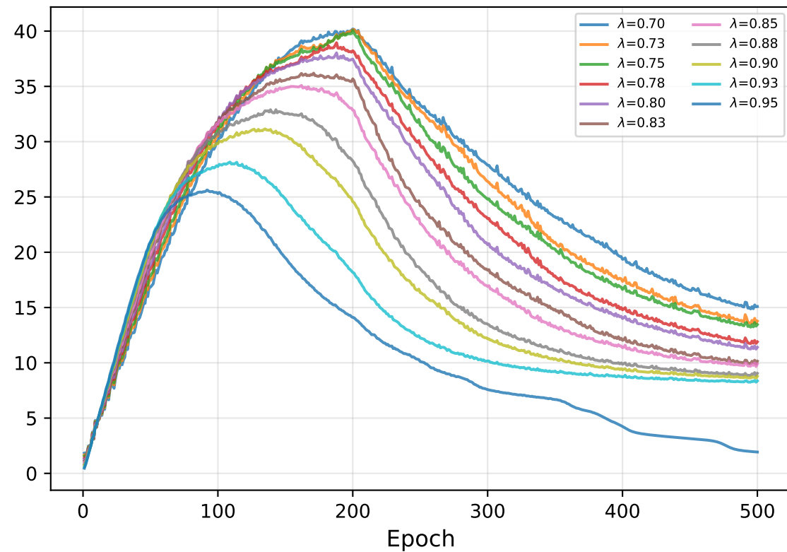
Total Loss
