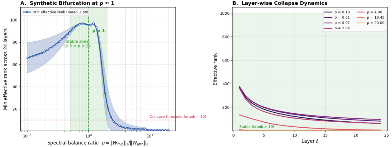
Figure 4: Synthetic bifurcation. (Left) Minimum effective rank vs. \rho across 24 layers; the stable zone is shaded. (Right) Layer-wise trajectories. Balanced \rho preserves high rank; imbalanced \rho collapses to \approx 1 .
