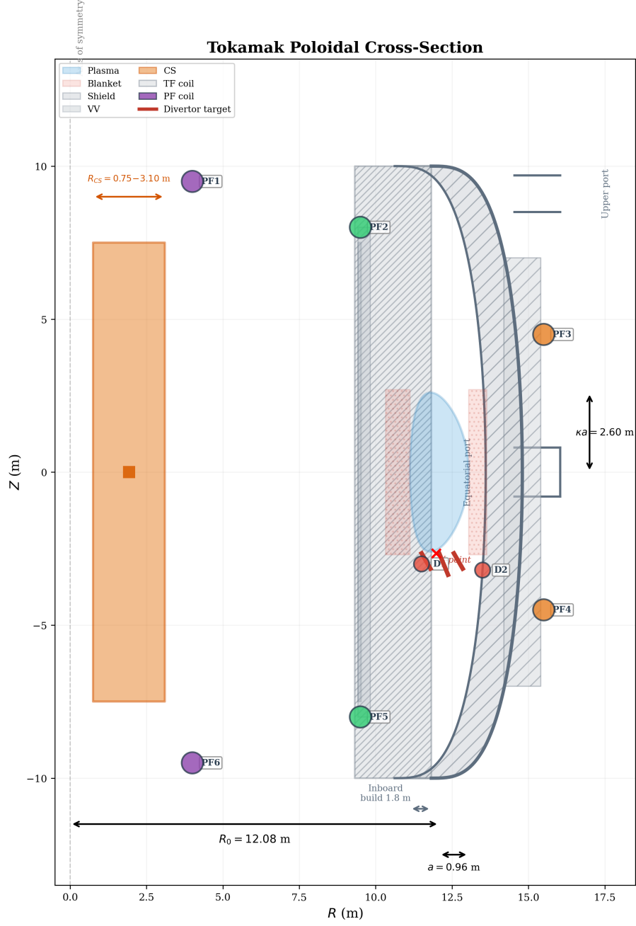
Figure 1: Poloidal cross-section of the reference design showing the major components: central solenoid (CS), toroidal field coils (TF), poloidal field coils (PF1–PF6, D1–D2), plasma, blanket, shield, vacuum vessel (VV), and snowflake divertor targets. Dimensions are labeled in meters.
