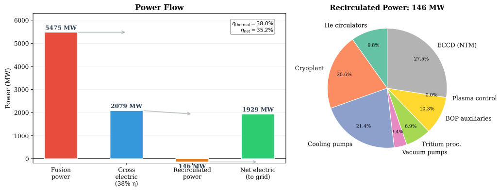
Figure 2: Power flow diagram. Left: waterfall chart showing fusion power (5,475 MW), gross electric (2,079 MW at 38% efficiency), recirculated power (146 MW), and net electric output (1,929 MW). Right: breakdown of recirculated power. The engineering gain is Q_{\text{eng}} = 13.3 .
