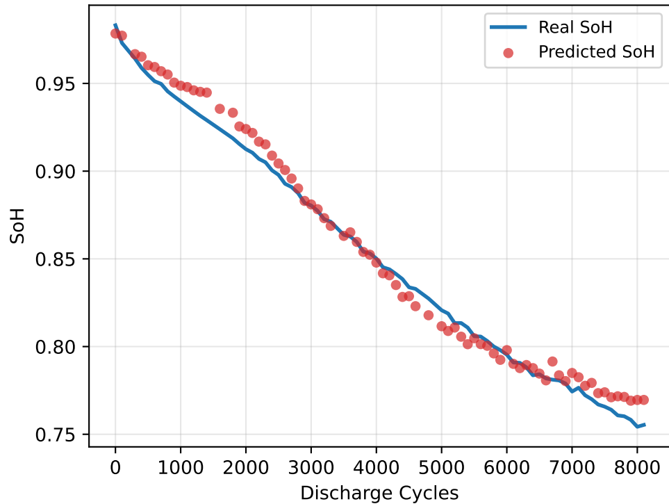
Fine-Tuned
