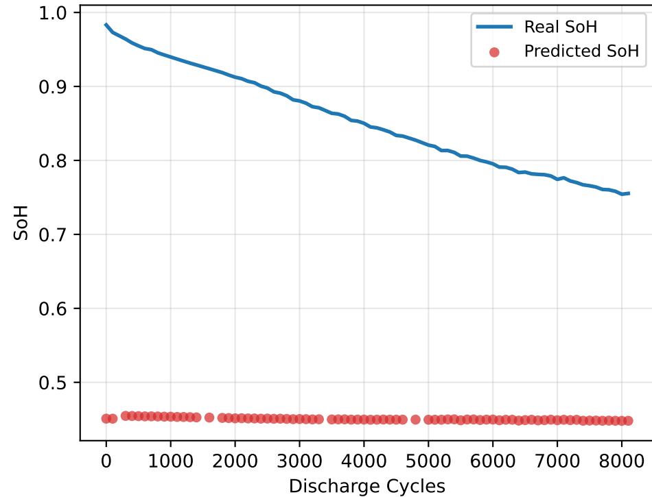
Zero-Shot
