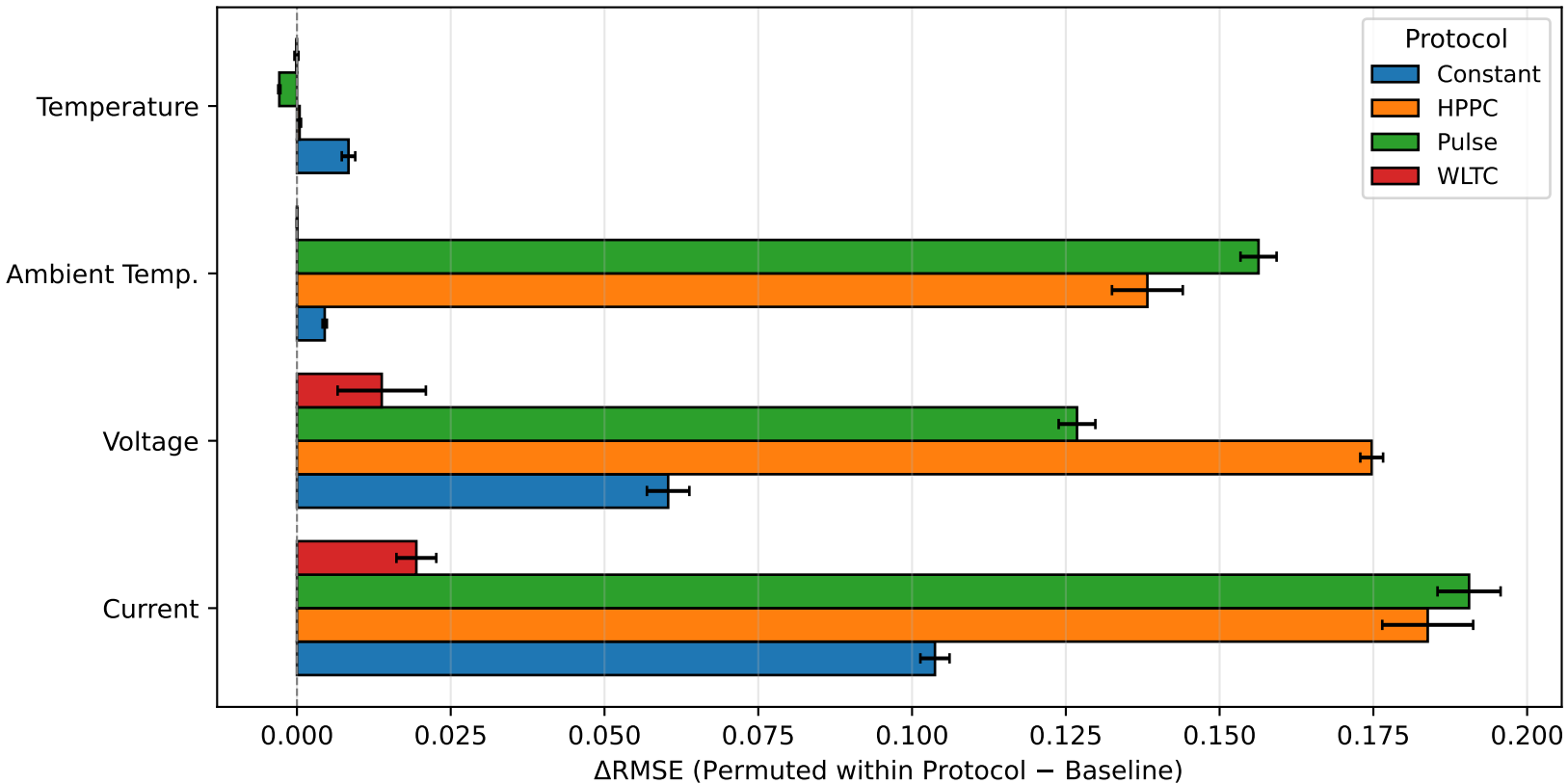
Stratified Permutation Feature Importance
