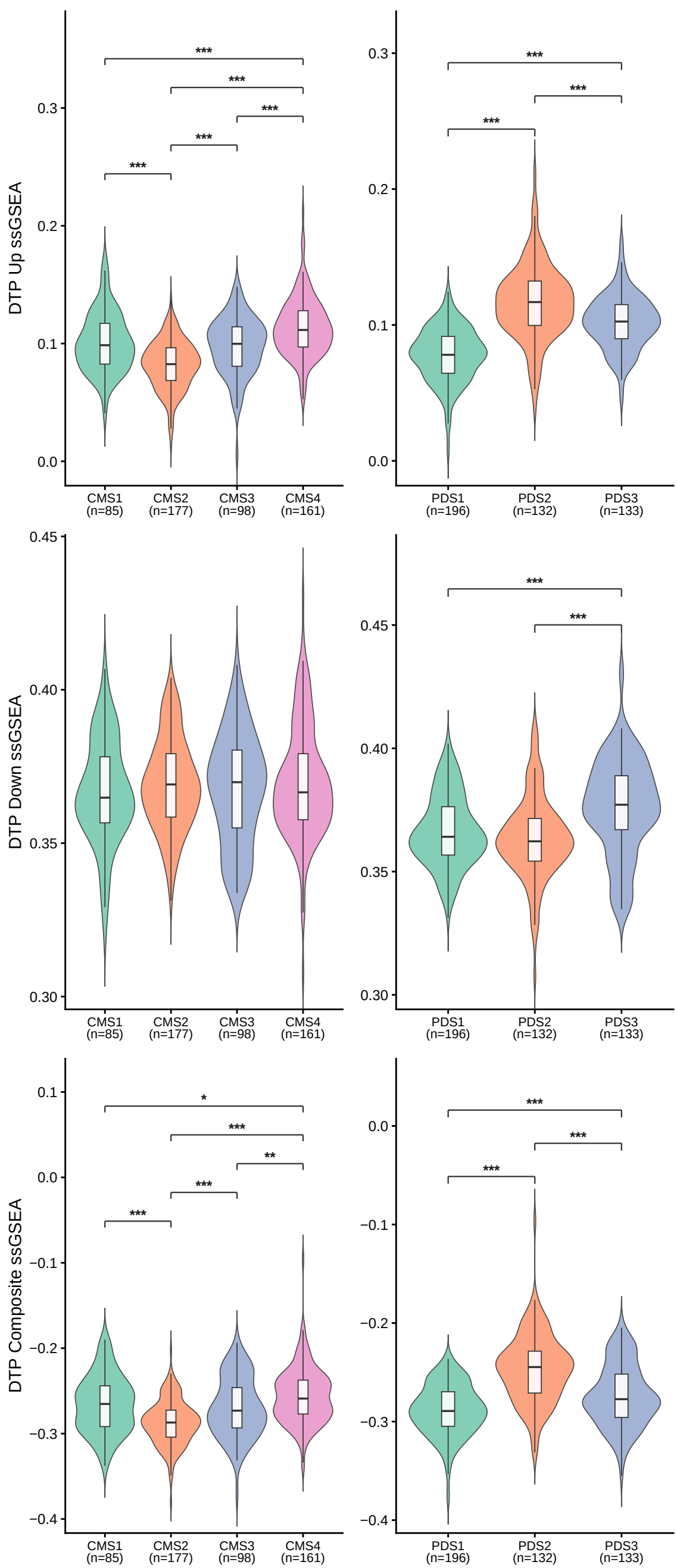
(A) Marisa (GSE39582); (B) TCGA-COAD. CMS and PDS subtype axes within each panel. CMS-unclassified and PDS "Mixed" are excluded. Pairwise Mann-Whitney tests with rank-biserial r, BH-corrected within each cohort x axis x score; only FDR<0.05 pairs are bracketed. Full pairwise table: Table_3_3C_subtype_pairwise.csv.
