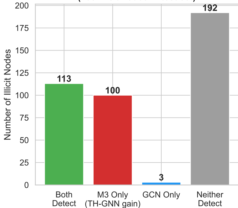
Detection Comparison (408 illicit nodes in test set)
