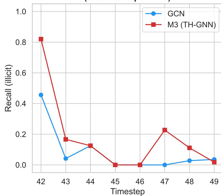
Per-Timestep Recall (test timesteps 42-49)
