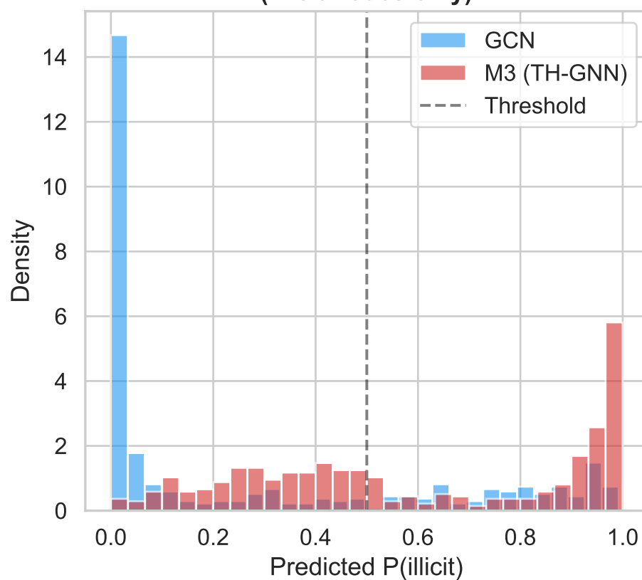
Prediction Distribution (illicit nodes only)
