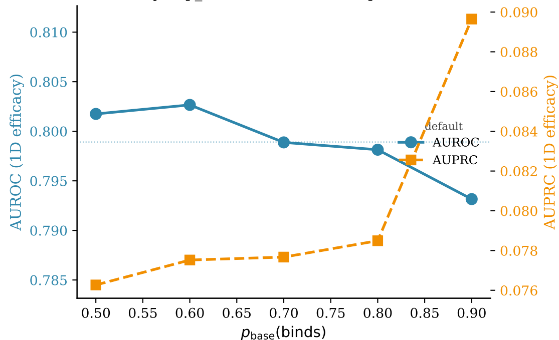
Sensitivity to p_{\text{base}}(\text{binds}) : AUROC spread = 0.0095
