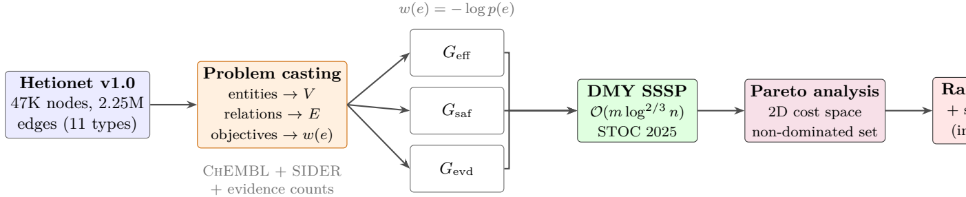
Figure 1: End-to-end framework. A biomedical knowledge graph (left) is cast into three parallel weighted directed graphs, one per clinical dimension (efficacy, safety, evidence), using a probability-to-distance transformation w(e) = -\log p(e) . Shortest-path distances computed by the DMY algorithm [Duan et al., 2025] give a D -dimensional cost vector per drug–disease pair, from which Pareto analysis selects non-dominated candidates. Each ranked drug is accompanied by an interpretable biological path through the knowledge graph.
