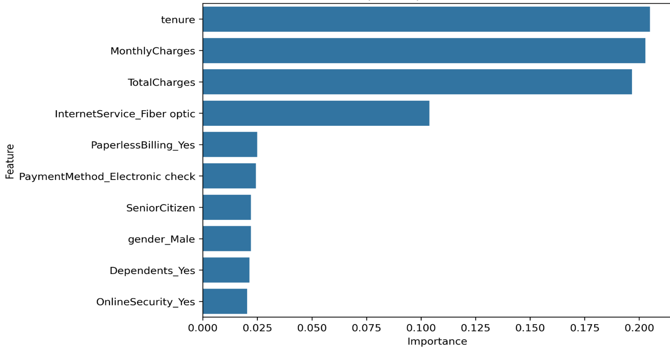
Top 10 Important Features
