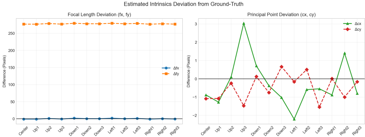
Figure 14: Intrinsic parameter deviations from ground truth for the initial calibration.
