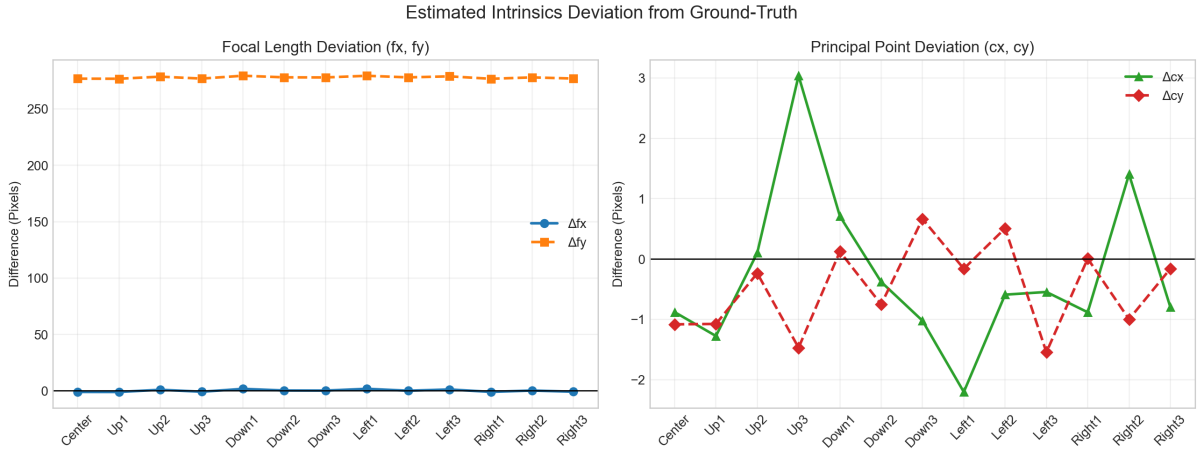
Figure 14: Intrinsic parameter deviations from ground truth and the initial calibration.
