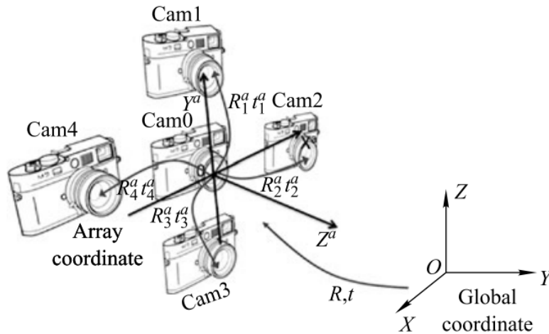
Figure 7: Representation of a multi-camera system. Source: [19].
