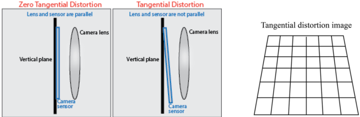
Figure 3: Visualization of tangential distortion. Source: [12], [11].
