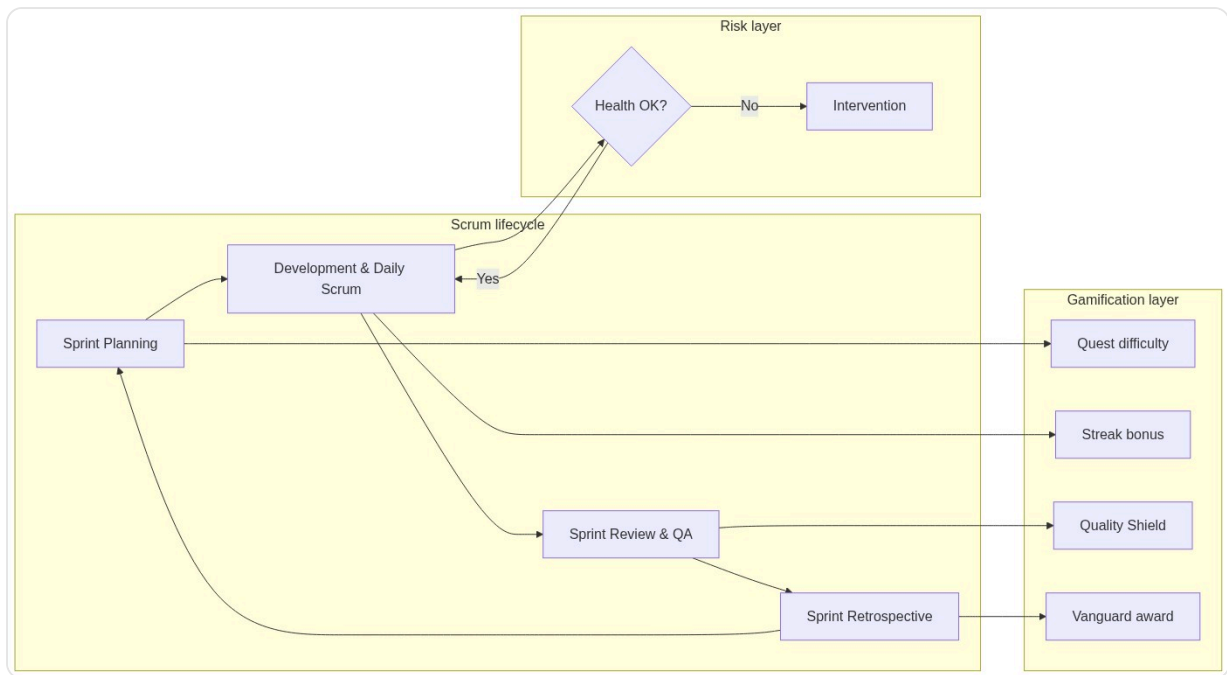
Figure 1 — Scrum lifecycle with gamification and risk layers
