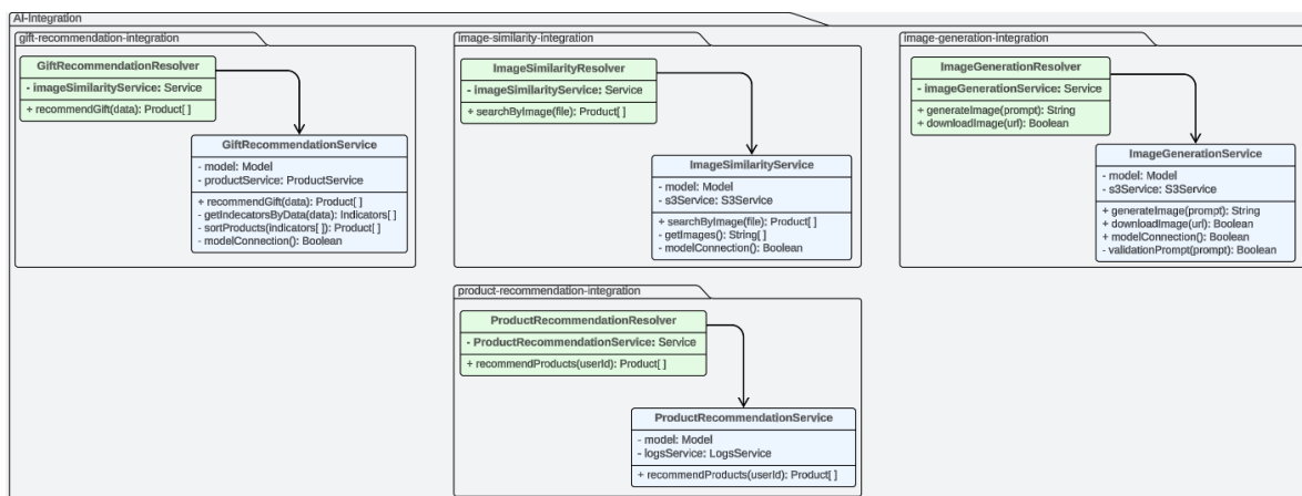
Figure 32: AI Integrations Class Diagram
