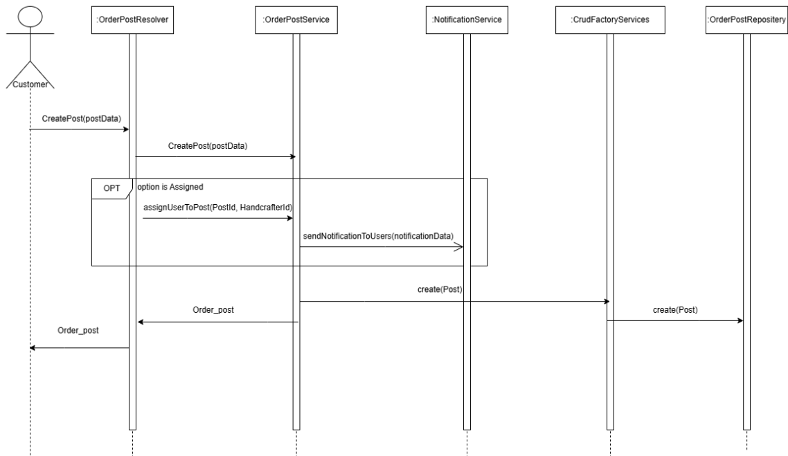
Figure 37: Add Post Sequence Diagram
