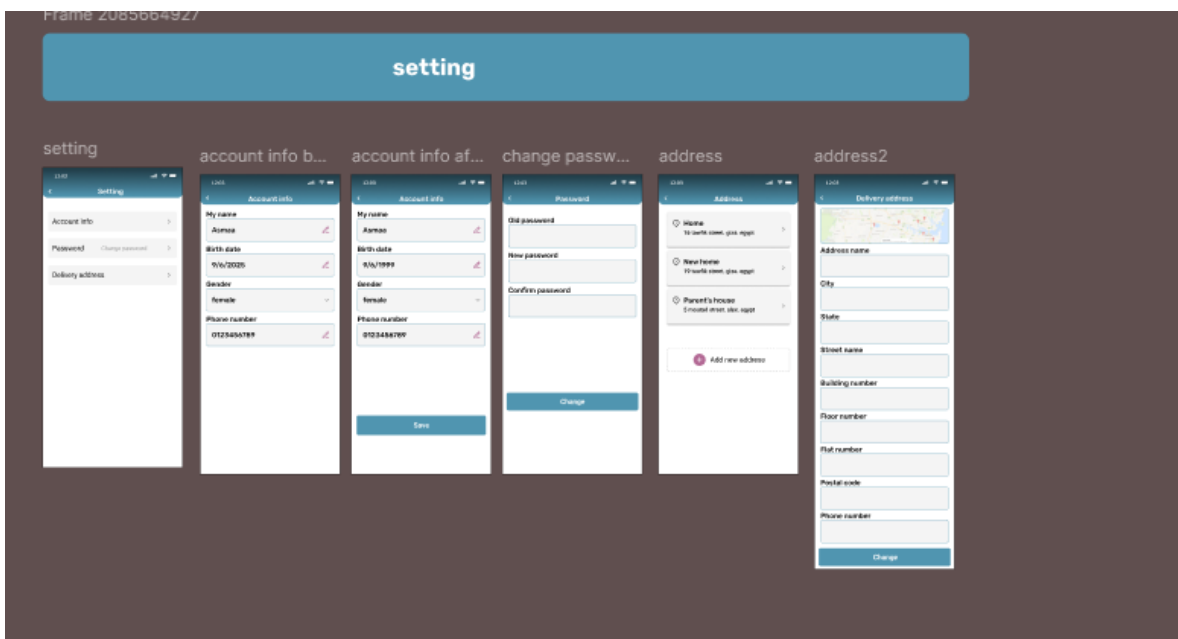
Figure 49: Figma UI
